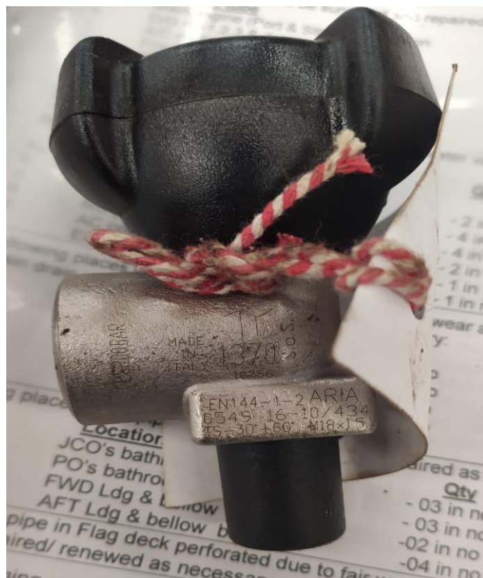
Figure-2: Pressure relief valve for BASCCA bottle (CPF 25.112 SL No.8)
